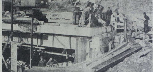
WORKMEN POUR CONCRETE at the Hudson Avenue Bridge over Mamaroneck River as the widening of the structure nears completion. The project is being conducted under the supervision of the Works Projects Administration, Westchester County.
